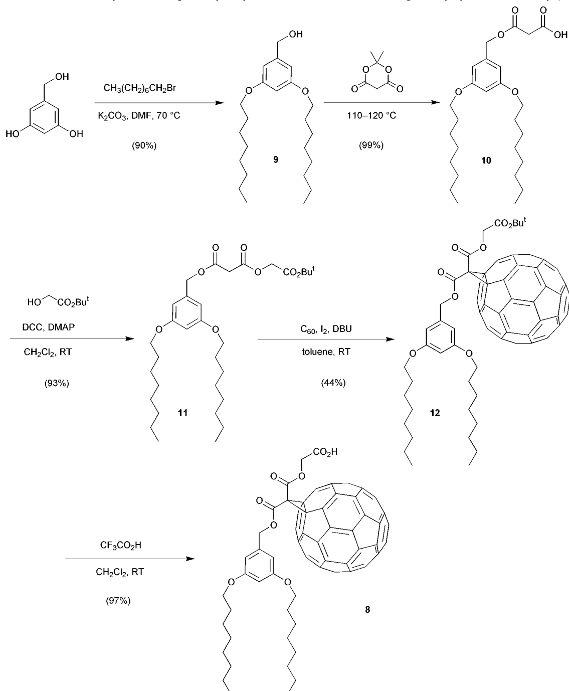
Scheme 2 Preparation of methanofullerene 8 (35% overall yield from 3,5-dihydroxybenzyl alcohol).
