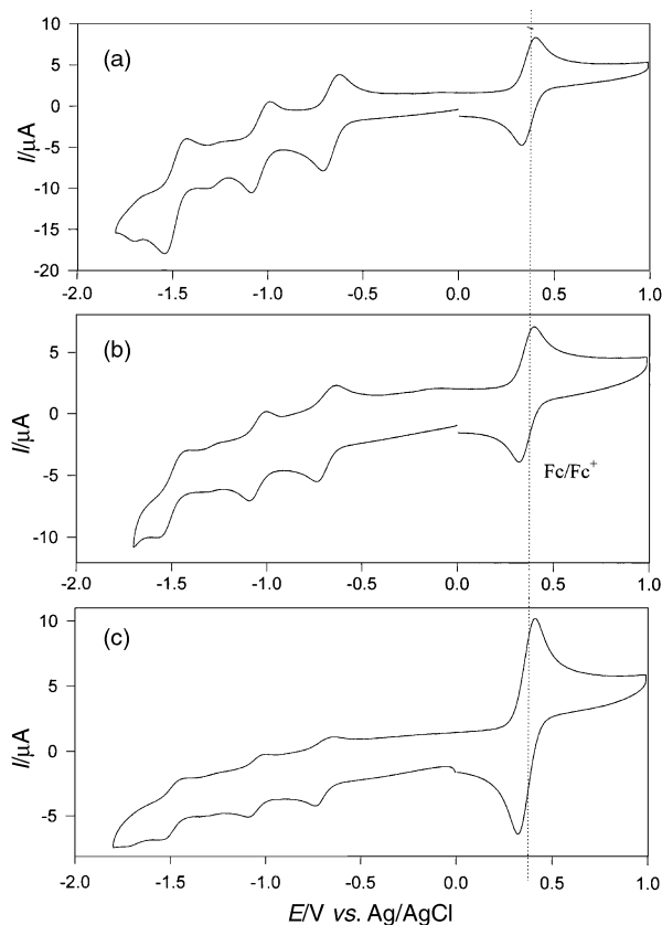
Fig. 1 Cyclic voltammetry of fullerodendrons (a) 12, (b) 13 and (c) 15 on a glassy carbon electrode at v = 0.1 \text{ V s}^{-1} in \text{CH}_2\text{Cl}_2 + 0.1 \text{ M Bu}_4\text{NPF}_6 in the presence of ferrocene used as internal reference.
