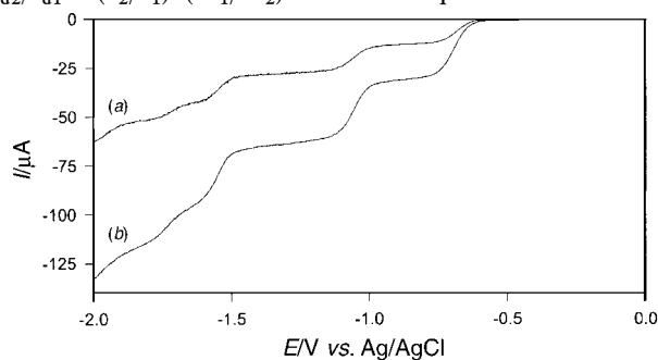
Fig. 2 SSV of (a) 12 and (b) 13 recorded at the same concentration ( 0.39 \text{ mmol L}^{-1} ) in \text{CH}_2\text{Cl}_2 + 0.1 \text{ M Bu}_4\text{NPF}_6 on a glassy carbon rotating electrode ( \omega = 209 \text{ rad s}^{-1} ).
