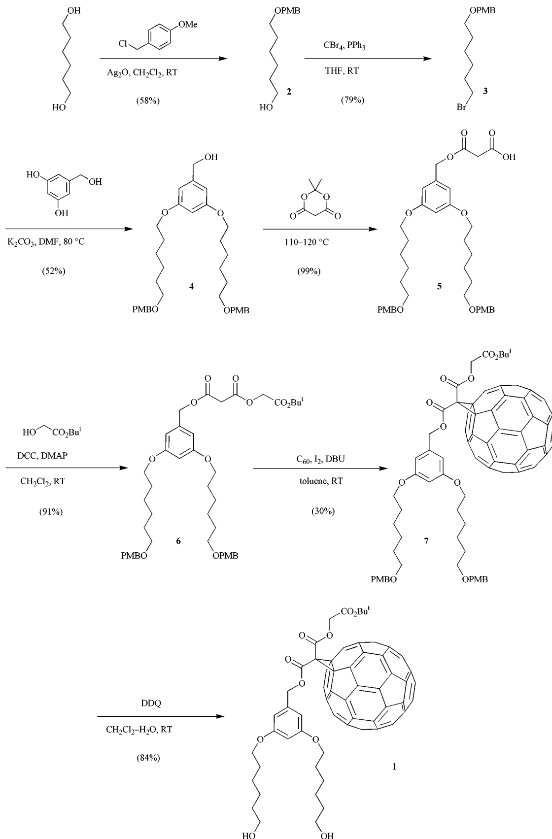
Scheme 1 Preparation of methanofullerene 1 (5% overall yield from 1,6-hexanediol).
