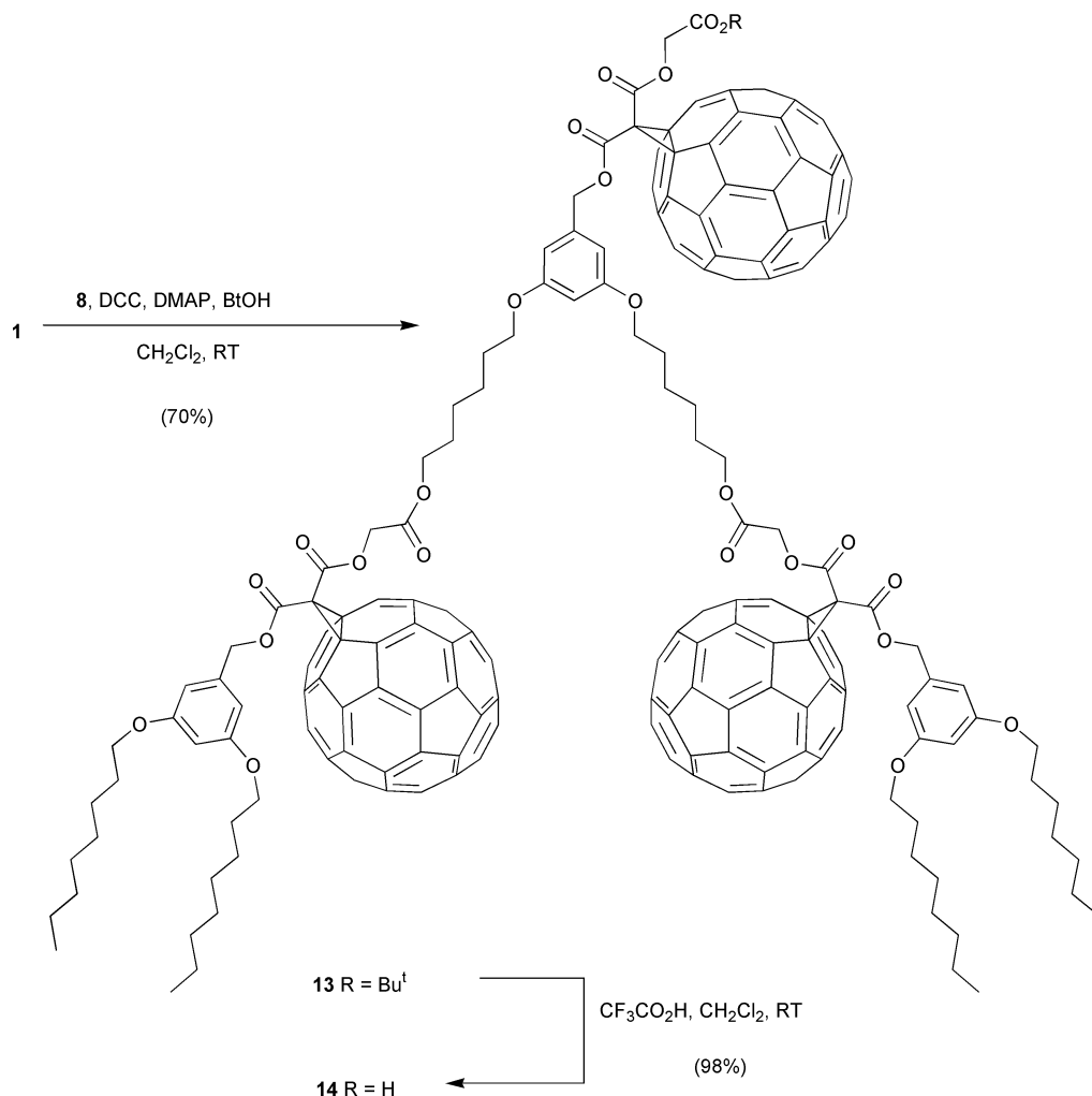
Scheme 3 Preparation of fullerodendron 14 .
