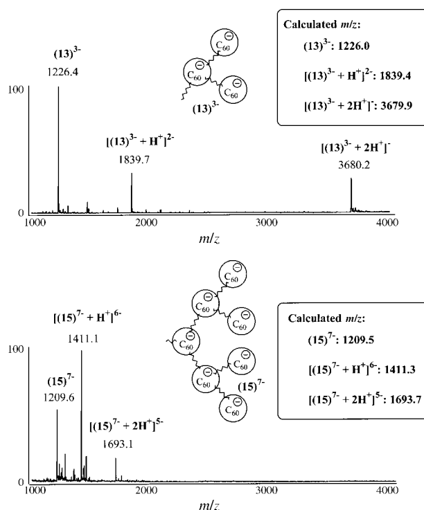
Fig. 4 ES mass spectra of 13 (top) and 15 (bottom).
