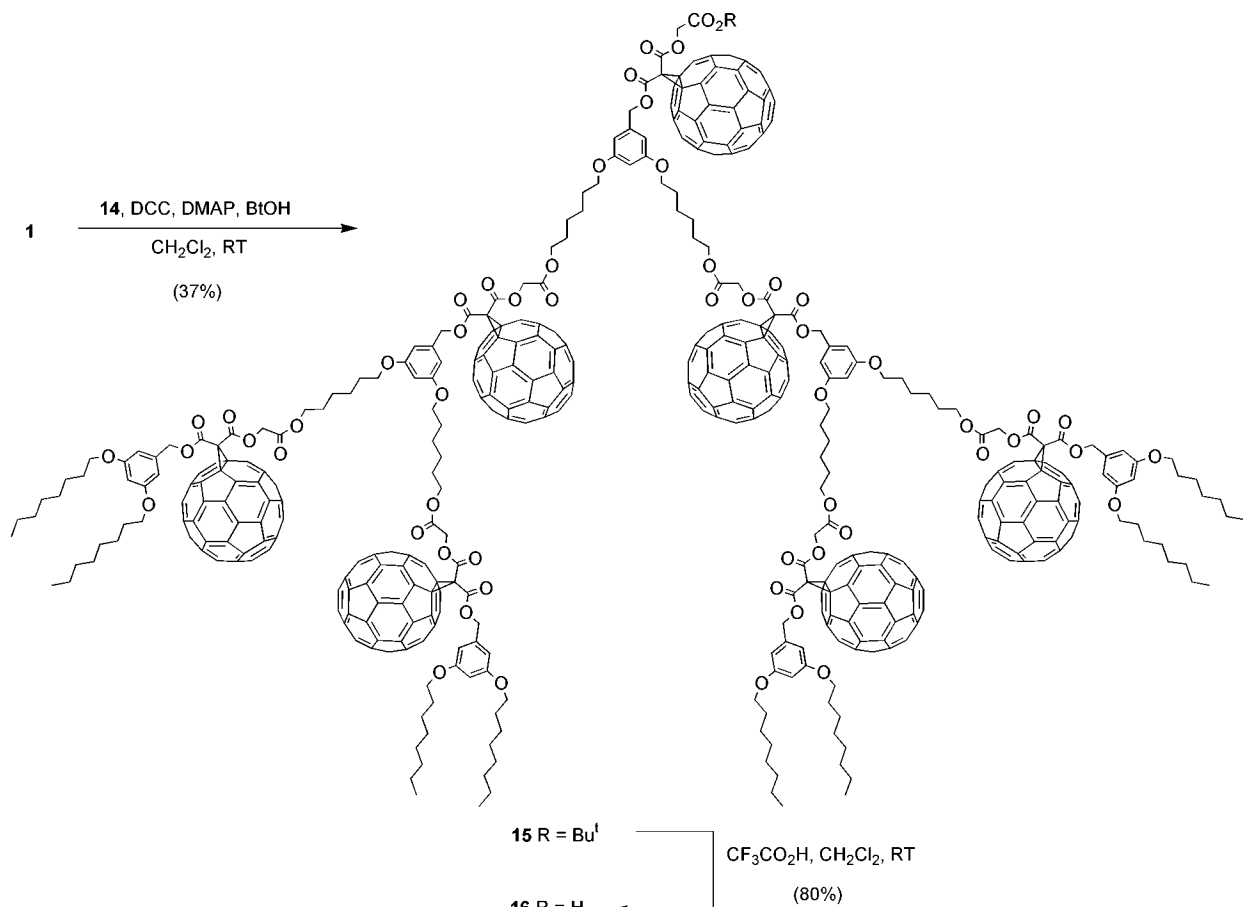
Scheme 4 Preparation of fullerodendron 16.
