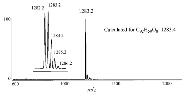
Fig. 3 ES mass spectrum of 12 recorded in the negative mode; the inset shows the isotopic pattern of the anion at m/z = 1283.2 .
